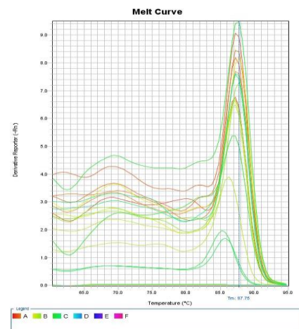
Figure 1. Melting curve of NLRP1 gene
